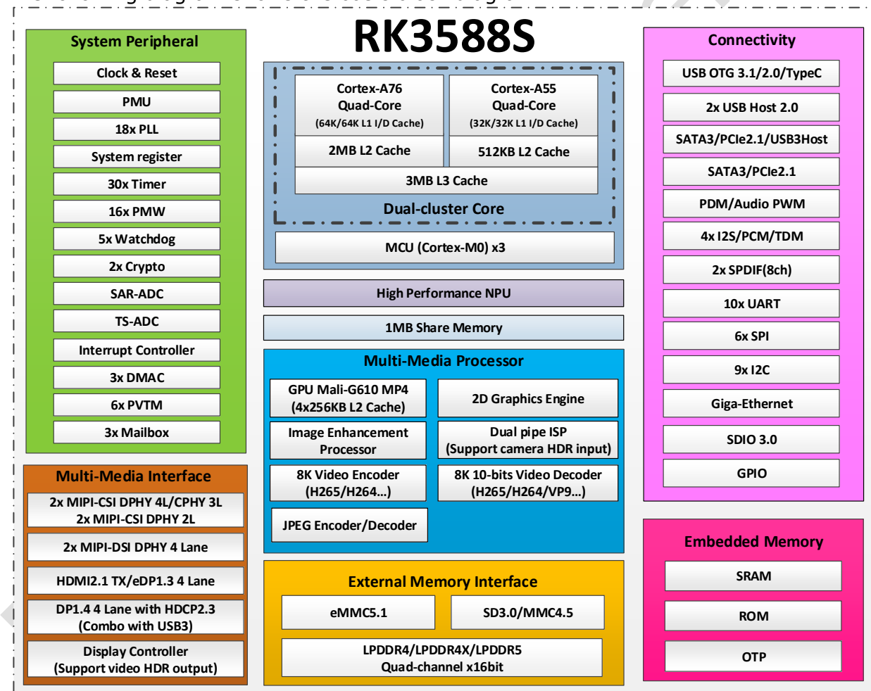
Fig.1-1 Block Diagram
